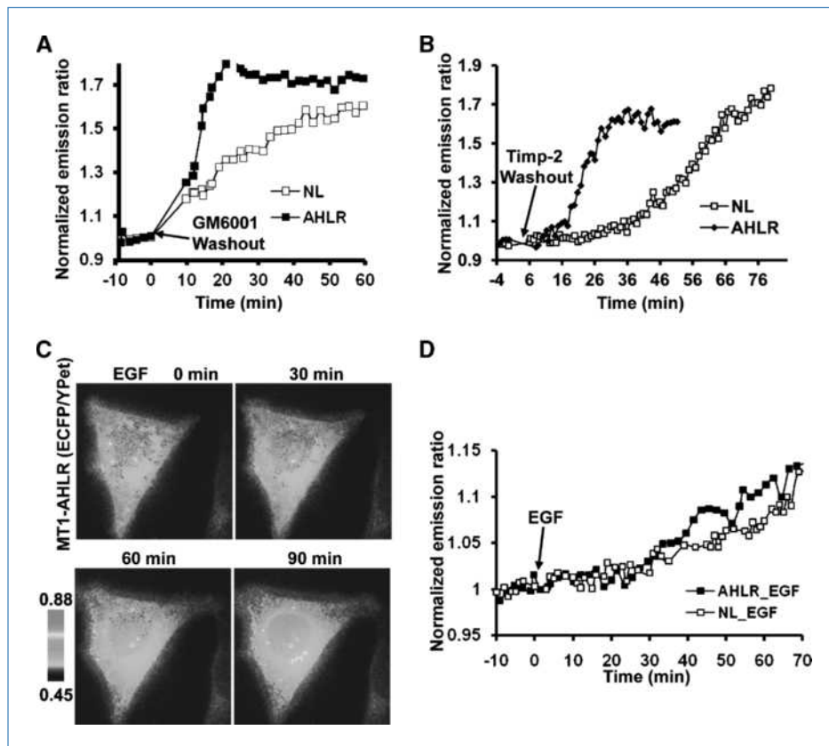
Figure 5. EGF induced a slow response of the optimized MT1-MMP biosensor. A and B, the ECFP/YPet emission ratio changes of the NL (□) and AHLR (■) biosensors in response to GM6001 (A; 5 μmol/L) or TIMP-2 (B; 100 nmol/L) for 12 h, followed by the washout with HBSS or acid/neutralization solutions, respectively. C, representative ECFP/YPet emission ratio images of the optimized AHLR FRET biosensor upon EGF stimulation in HeLa cells expressing MT1-MMP. D, the ECFP/YPet emission ratio time courses of the NL (□) and AHLR (■) biosensors before and after EGF stimulation in HeLa cells expressing MT1-MMP.
