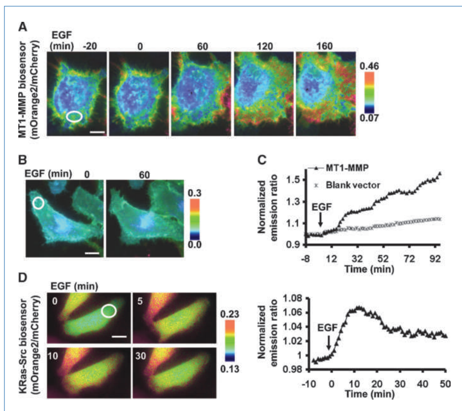
Figure 2. The characterization of mOrange2 and mCherry as a FRET pair in mammalian cells. A and B, representative mOrange2/mCherry emission ratio images of the MT1-MMP biosensor before and after EGF stimulation in HeLa cells expressing MT1-MMP (A) or a blank vector (B). C, representative time courses of normalized mOrange2/mCherry emission ratio of the MT1-MMP biosensor in HeLa cells expressing MT1-MMP (▲) or a blank vector (*). D, representative images (left) and time course of normalized mOrange2/mCherry emission ratio (right) in HeLa cells expressing the Src biosensor before and after EGF stimulation. Bars, 30 \mu m.
