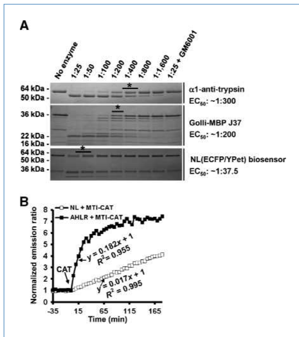
Figure 4. The development of an optimized MT1-MMP biosensor. A, the comparison of cleavage speeds of three MT1-MMP substrates (AAT, MBP-J37, and the NL ECFP/YPet biosensor) by MT1-CAT. MT1-CAT was incubated with the different substrate proteins at 1:25 to 1:1,600 molar ratios for 3 h at 37°C. *, the ratio condition that half of the substrate was cleaved. Right, the corresponding EC_{50} value. B, comparison of the cleavage speed of the purified NL (□) and AHLR (■) biosensors. The time courses show the normalized emission ratio (ECFP/YPet) change of biosensors (1 \mu mol/L) before and after the addition of MT1-CAT (2 \mu g/mL). The equations and R^2 values represent the initial slopes of the emission curves upon MT1-CAT incubation.
