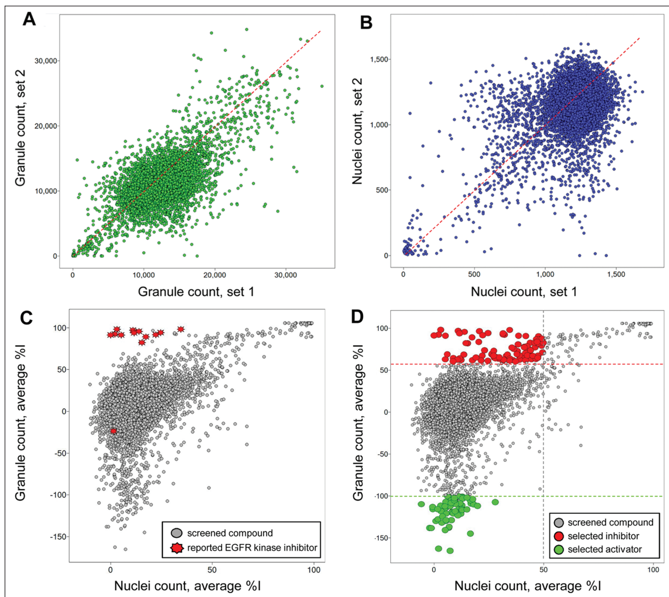
Figure 3. Scatter plot analysis of the pilot screen performed in duplicate. A library of 6912 compounds was screened in duplicate to evaluate assay reproducibility and performance. (A) The granule count for each compound and for each set of data is plotted as a scatter plot, demonstrating the reproducibility of the granule count readout during the pilot screen. (B) The nuclei count for each compound and for each set of data is plotted as a scatter plot, demonstrating the reproducibility of the nuclei count readout during the pilot screen. (C, D) The average percentage inhibition in the granule count for each compound for both replicate sets of data is plotted against the average percentage inhibition in the nuclei count of each compound for positive selection. (C) Twelve of 13 reported epidermal growth factor receptor (EGFR) kinase inhibitors are clustered in the scatter plot, inducing a high percentage inhibition in granule count and low percentage in nuclei count. (D) Positives for inhibition of granule formation in the pilot screen are selected as those compounds inducing greater than 60% inhibition of granule formation and less than 50% inhibition in nuclei count. Activators of granule formation in the pilot screen are selected as those compounds inducing lower than -100% inhibition of granule formation and lower than 50% inhibition in nuclei count.
