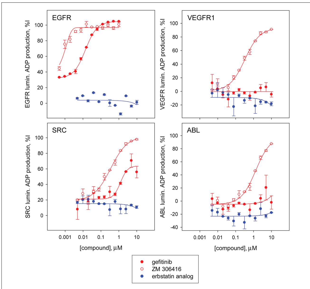
Figure 5. Assessment of potency of selected hits in a panel of kinases using the luminescence adenosine diphosphate (ADP) production kinase assay. Dose-response studies of gefitinib, ZM-306416, and the erbstatin analog against a kinase panel consisting of the kinases EGFR, VEGFR1, SRC, and ABL. The epidermal growth factor receptor (EGFR) kinase inhibitor gefitinib is selectively potent toward EGFR, with a calculated \text{IC}_{50} of <0.01 \mu\text{M} , and low or no activity toward VEGFR1 ( \text{IC}_{50} > 10 \mu\text{M} ), SRC ( \text{IC}_{50} > 10 \mu\text{M} ), and ABL ( \text{IC}_{50} > 10 \mu\text{M} ). In contrast, ZM-306416 is potent toward all kinases of the panel: EGFR ( \text{IC}_{50} < 0.01 \mu\text{M} ), VEGFR1 ( \text{IC}_{50} = 0.33 \pm 0.04 \mu\text{M} ), SRC ( \text{IC}_{50} = 0.33 \pm 0.08 \mu\text{M} ), and ABL ( \text{IC}_{50} = 1.3 \pm 0.2 \mu\text{M} ). Erbstatin analog is inactive ( \text{IC}_{50} > 10 \mu\text{M} ) toward all kinases in the panel, including EGFR kinase.
