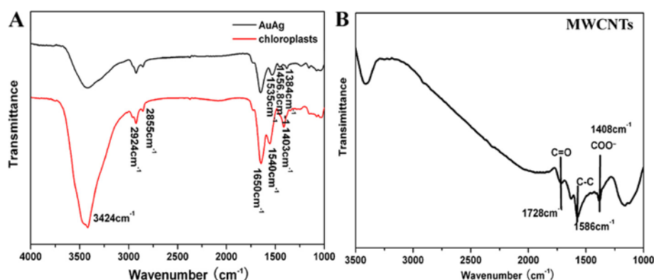
Figure 4 (A) FTIR spectra of chloroplasts and Au-Ag alloy scanning at a range of 4,000 to approximately 1,000 \text{cm}^{-1} ; (B) FTIR spectra of acid-treated MWNTs.
