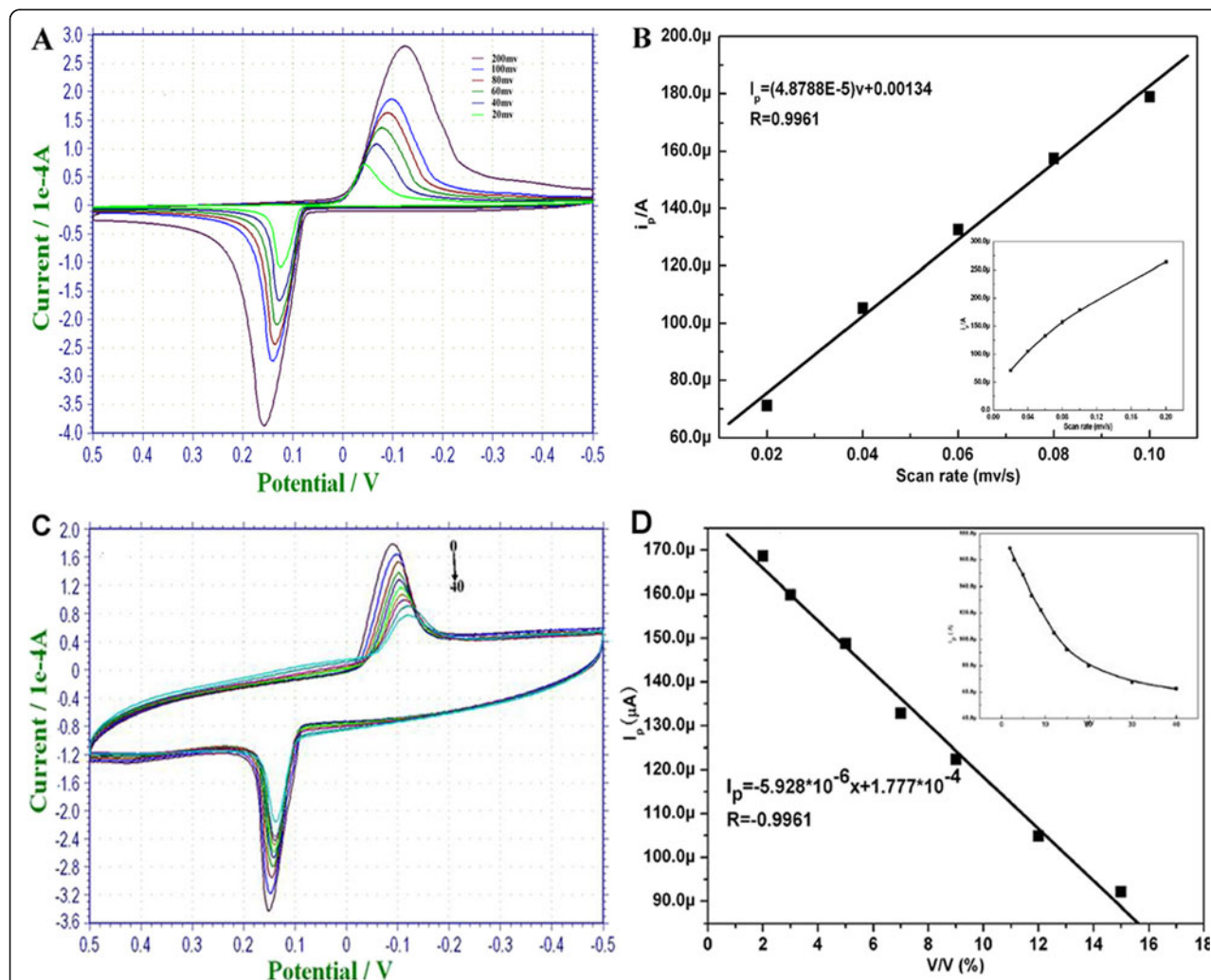
Figure 6 The performance of cyclic voltammograms. (A) Cyclic voltammograms of the Au-Ag/MWNT working electrode at various scan rates from 20 to 200 mV/s in 0.1 -mol/L KCl solution. All potentials are given versus SCE; (B) displays the dependence of the redox peak currents ( I_p ) on the scan rates ( \nu ). The inset shows redox peak currents plot with scan rate at a range of 20 to approximately 200 mV/s. (C) Cyclic voltammograms of Au-Ag/MWNTs/GCE were exposed to various concentrations of 2-butanone at ranges of 0\% to approximately 20\% (v/v) in 0.1 -M KCl solution; (D) the linear calibration plot of the peak current against butanone. The inset shows the curve of the peak current corresponding to different concentrations of 2-butanone.
