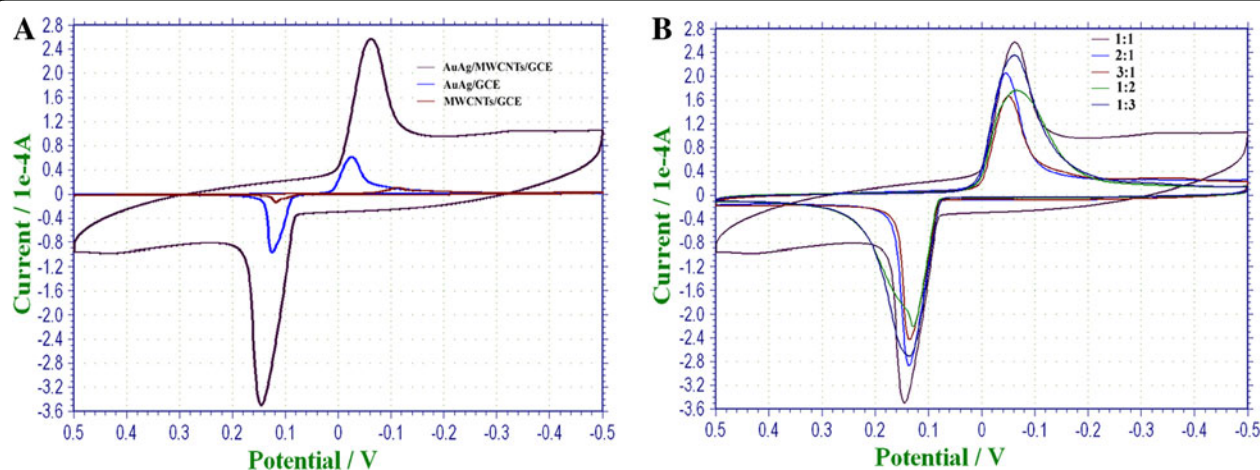
Figure 5 The amperometric response of Au-Ag/MWNT working electrode. (A) Curves of CV were obtained with different working electrodes (MWNTs/GCE, Au-Ag/GCE, and Au-Ag/MWNTs/GCE); (B) the amperometric response of Au-Ag/MWNT working electrode with different molar ratios between Au-Ag and MWNTs (3:1, 2:1, 1:1, 1:2, and 1:3, respectively).
