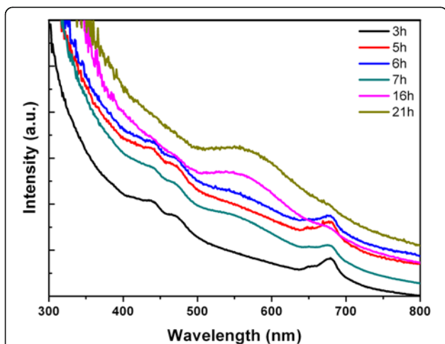
Figure 1 UV-vis spectra. The UV-vis spectra were recorded as a function of reaction time in the range of 300 to 800 nm, when equimolar ratio of \text{HAuCl}_4 and \text{AgNO}_3 were introduced into the chloroplast solution. The time intervals are 3, 5, 6, 7, 16, and 21 h.
