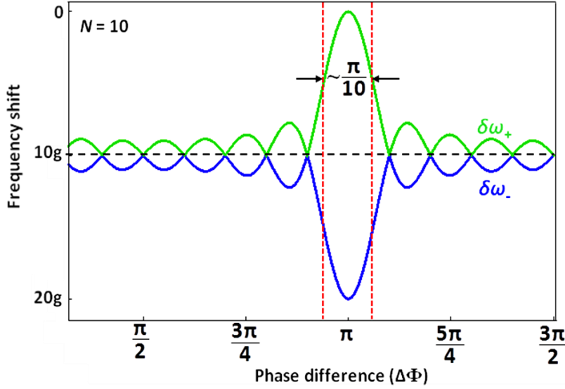
Fig. 4. Variation of the frequency shift of the WGM in the presence of 10 epitopes adsorbed on a microcavity as a function of phase difference between the consecutive epitopes.
