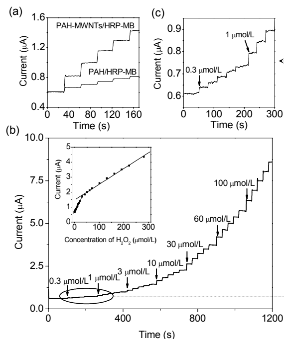
Fig. 6 Current responses of Au electrodes
