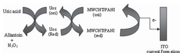
Figure 3. Scheme of electron flow and current generation in uric acid biosensor employing Uricase/MWCNT/PANI/ITO electrode.
