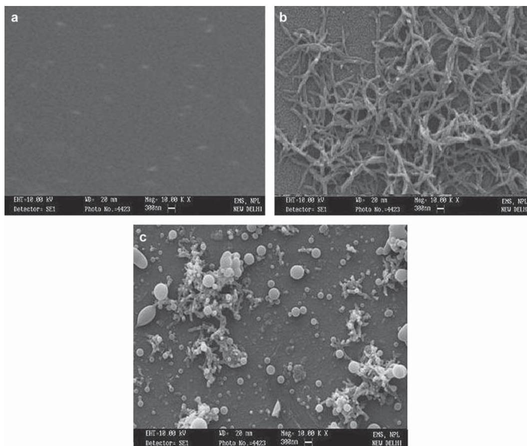
Figure 2. (2a) Scanning electron micrographs of PANI deposited on ITO coated glass plate (2b) Scanning electron micrographs of MWCNT/PANI deposited on ITO coated glass plate (2c) Scanning electron micrographs of MWCNT/PANI/uricase deposited on ITO coated glass plate.
