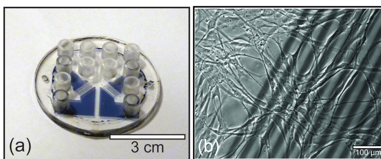
Figure 4. Cell-based biosensor. (a) All polymer microdevice with two functional channels fabricated in TOPAS (uncolored) and PEDOT:TsO (blue). (b) Healthy cells cultured on PEDOT:TsO microelectrodes in the biosensor.
