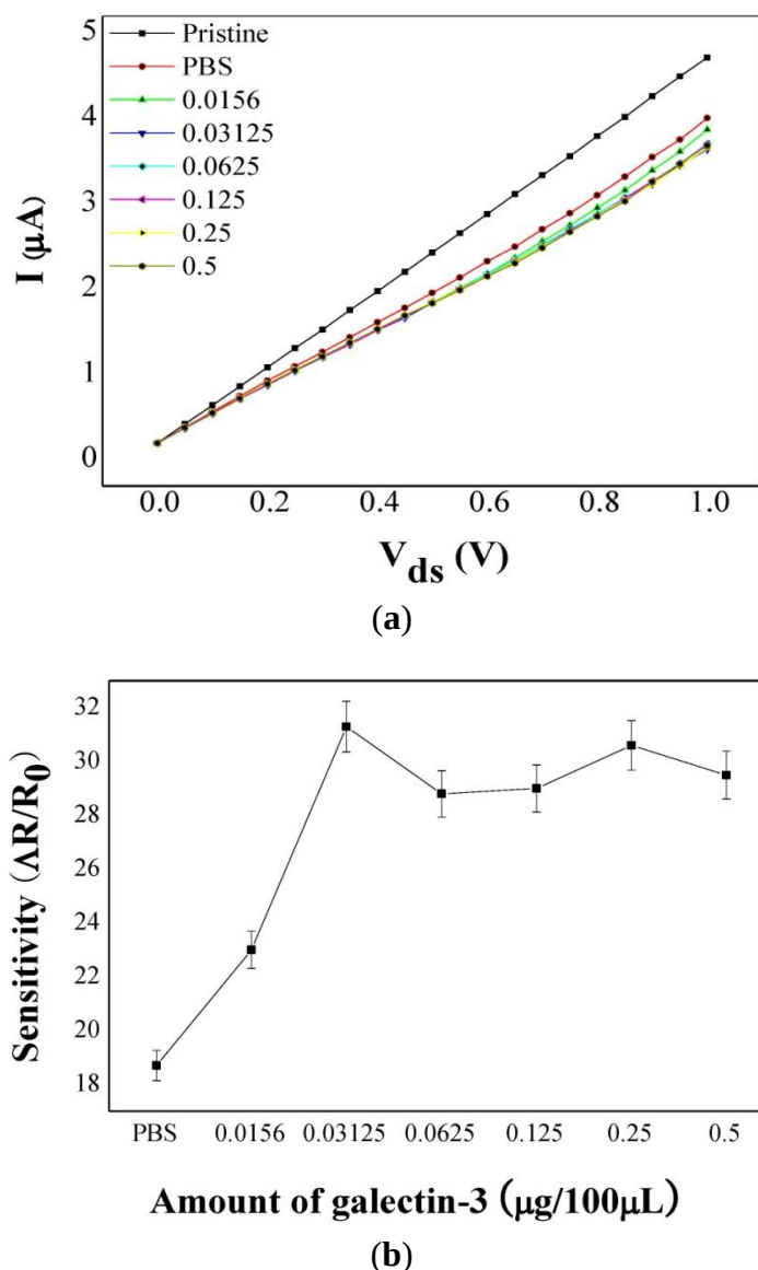
Figure 4. Typical graphical data for (a) I-V measurements and (b) the sensitivities of samples with or without galectin-3. The typical I-V characteristics were measured using the prepared Mo electrodes. SWCNTs dispersed between the Mo electrodes were exposed to various concentrations of galectin-3 in PBS (two-fold serial dilutions from 0.5 to 0.0156 \mu\text{g}/100\text{ }\mu\text{L} ). The results were obtained from three different experiments. Each bar represents the mean standard deviation.
