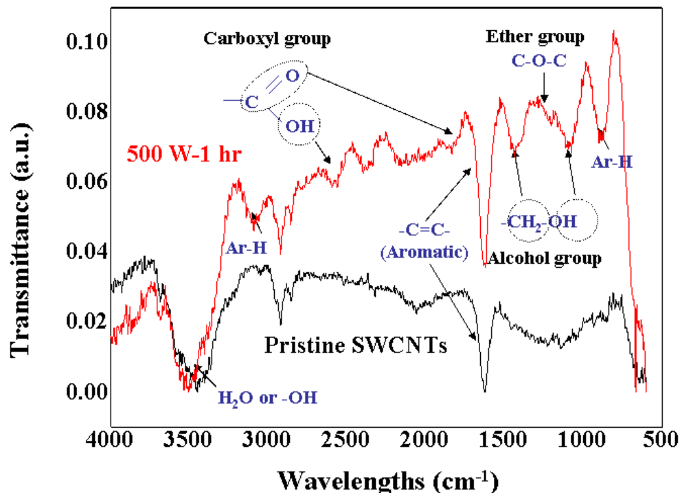
Figure 2. FT-IR analysis after introducing D-(+)-galactose on the surface of SWCNT-COCl. The stretching frequencies of ether and alcoholic linkages (C–O–C, –CH 2 –O) were seen around 1000~1300 cm −1 , the carbonyl of carboxylic acid at ~1700 cm −1 , and the –OH of carboxylic acid at ~2500 and ~3500 cm −1 .
