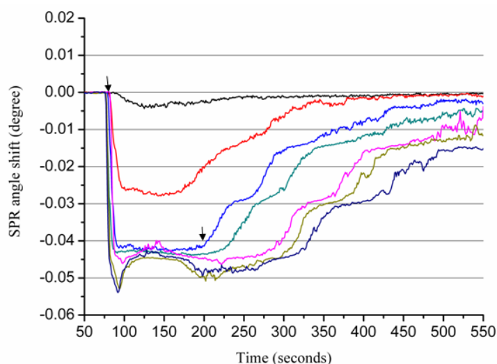
Figure 2. The sensorgrams for the interactions between \text{Zn}^{2+} ions and the \text{A}\beta_{1-28} peptides. Various concentrations (50, 100, 200, 300, 600, 700 and 800 \mu\text{M} , from top to bottom) of \text{Zn}^{2+} ions were injected onto the \text{A}\beta_{1-28} sensorchip. Arrows indicate \text{Zn}^{2+} ions starting to flow onto immobilized \text{A}\beta_{1-28} and when the flowing of metal ions ends, respectively.
