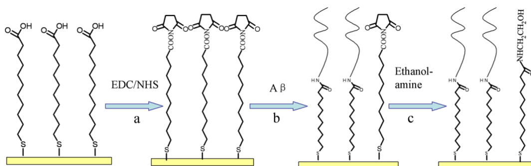
Figure 7. The procedure for the immobilization of A \beta . (a) The self-assembled monolayer (SAM) of MUA surface was activated with standard amine coupling chemistry using EDC/NHS; (b) The activated surface was covered with a fresh A \beta solution to form a bond between the amine group on the peptide and the carboxylic group on the MUA surface; (c) The remaining activated surface groups were blocked using ethanolamine.
