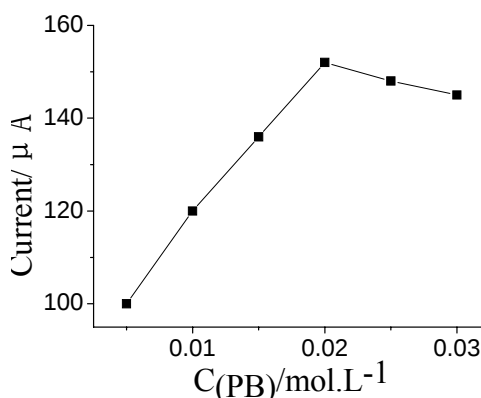
Figure 6. Effect of the concentration of PB in Nf membrane on DPV current. DPV conditions: 25 \text{ }\mu\text{L} \text{pH} = 7.5 \text{KNO}_3 solution contain 1.0 \text{ mmol}\cdot\text{L}^{-1} ATCh and after the AChE was inhibited by OPs for 5 min at 35 \text{ }^\circ\text{C} .
