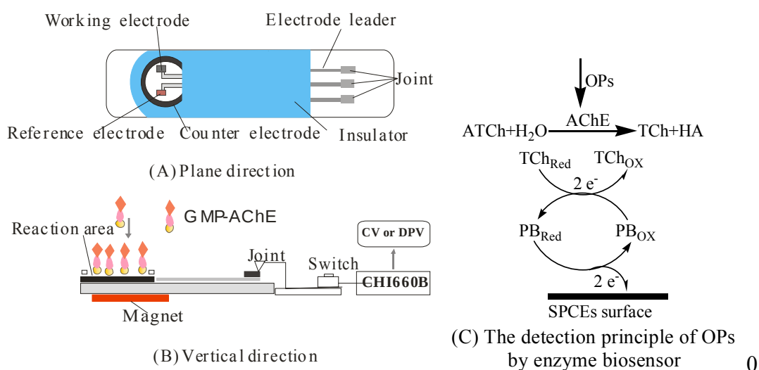
Figure 2. Preview of the enzyme biosensor apparatus from the plane (a), vertical direction (b), and the detection principle of OPs by the biosensor; (c) CV and DPV conditions: 25 \mu L pH = 7.5 KNO 3 solution contain 1 mmol·L -1 ATCh and the scanning potential range both were +0.6 \rightarrow -0.2 V.
