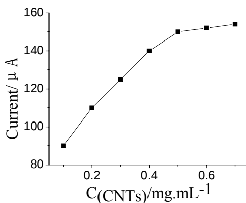
Figure 5. Effect of the concentration of CNTs in Nf membrane on DPV current. DPV conditions: 25 μL pH = 7.5 KNO 3 solution contain 1.0 mmol·L -1 ATCh and after the AChE was inhibited by OPs for 5 min at 35 °C.
