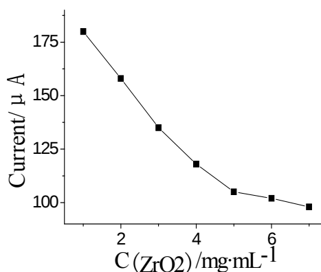
Figure 7. Effect of the concentration of \text{ZrO}_2 in Nf membrane on DPV current. DPV conditions: 25 \text{ }\mu\text{L} \text{pH} = 7.5 \text{KNO}_3 solution containing 1.0 \text{ mmol}\cdot\text{L}^{-1} ATCh and after the AChE was inhibited by OPs for 5 min at 35 \text{ }^\circ\text{C} .
