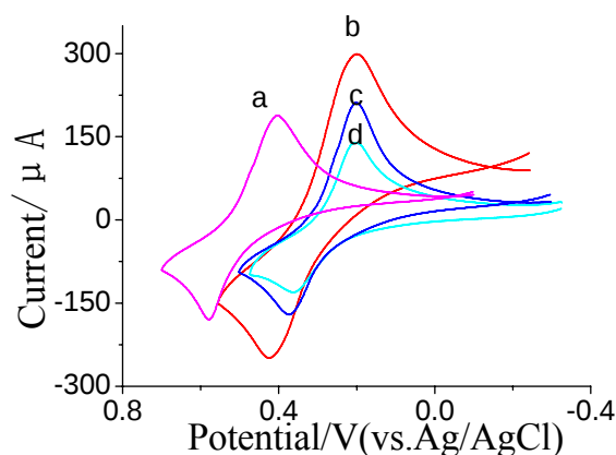
Figure 4. Cyclic voltammetry curves (CVs) of SPCE | CNTs/ZrO 2 /Nf | GMP-AChE (a), SPCE | CNTs/ZrO 2 /PB/Nf | GMP-AChE (b), SPCEs | ZrO 2 /PB/Nf | GMP-AChE (c), and c inhibited by 1.0 ng·mL -1 dimethoate for 5 min at 35 °C (d) in 1.0 mmol·L -1 ATCh + 0.1 mol·L -1 KNO 3 (pH = 7.5).
