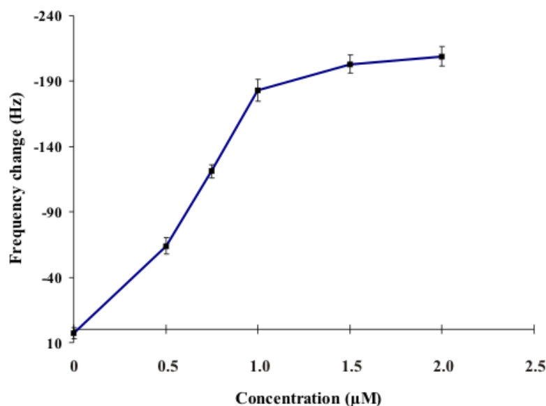
Figure 1. Resonant frequency changes of quartz crystal by thiol-modified oligonucleotide probe immobilization. Frequency changes were represented by the frequency differences between the frequency value of thiol-modified oligonucleotide probe immobilized on gold electrode (F1) and frequency value of original quartz crystal (F0) before immobilization ( \Delta F = F_0 - F_1 ). Each data point represents the mean \pm SD ( n = 3 ).
