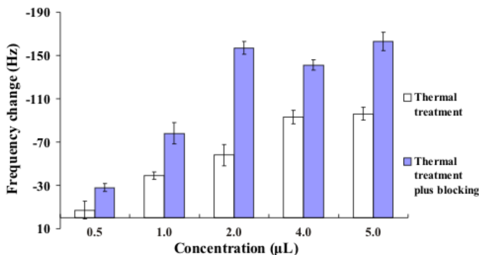
Figure 3. Resonant frequency change of DNA solution. BtgI ( Bst DSI)-digested IS6110 of M. tuberculosis genomic DNA was diluted with hybridization buffer before hybridization assay on piezoelectric biosensor. Each data point represents the mean \pm SD ( n = 3 ).
