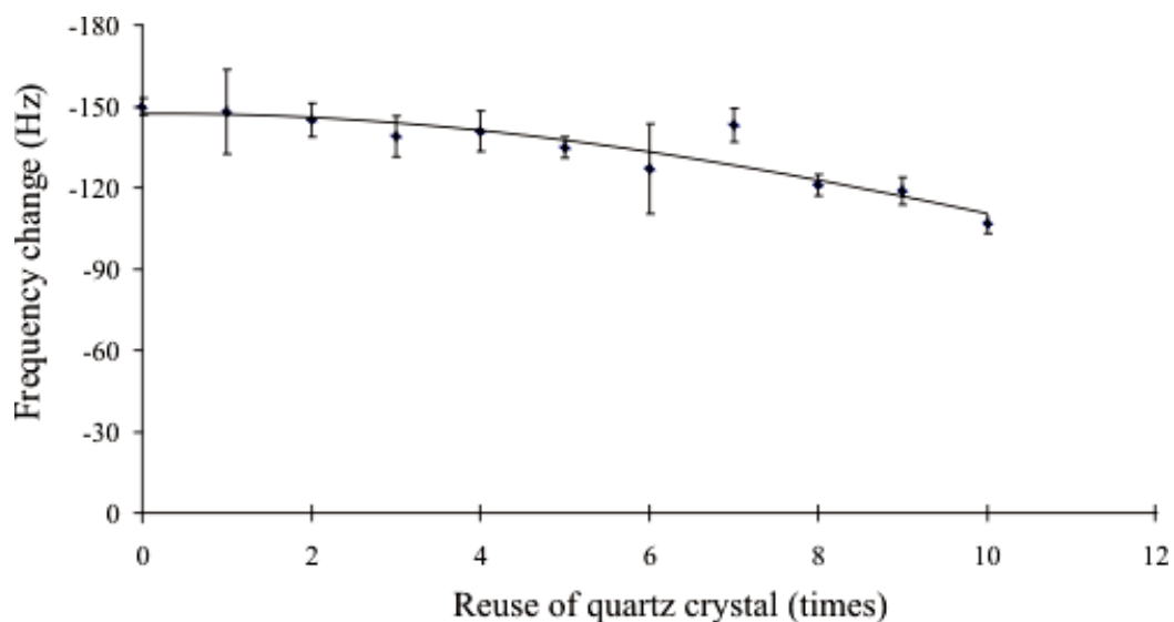
Figure 5. Resonance frequency change during testing of piezoelectric DNA-based biosensor reusability. 1.5 \mu\text{M} of synthetic DNA target was applied on the sensor at room temperature for 20 minutes to hybridize with probe. Each used sensor was added with 10 \mu\text{L} of 1mM HCl for one minute to wash out prior hybridized DNA target. The next cycle of hybridization was performed to test the capability of sensor. Each data point represents the mean \pm SD ( n = 3 ).
