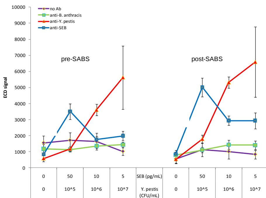
Figure 7. Two-plex assay for SEB and Y. pestis . Chips were incubated with 0, 10^5 , 10^6 , or 10^7 CFU/mL Y. pestis and 0, 5, 10, or 50 pg/mL SEB. Anti- B. anthracis , anti- Y. pestis , and anti-SEB refer to the antibodies immobilized on the chip surface. Mean signals and SD are indicated. Note: breaks in SEB line serve as a reminder that concentrations for all samples are not continuous and that lines are only used to illustrate trends.
