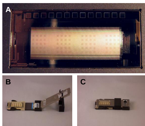
Figure 1. CombiMatrix antibody microarray (A) Arrays are subdivided into four identical sub-arrays divided into 20 discrete antibody blocks each; (B) Hybridization clamp that holds the chip and hybridization cap covering the microarray; (C) Fully assembled clamp, cap, and chip.
