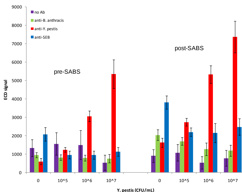
Figure 6. Y. pestis assay in 50% serum. Chips were incubated with 0, 10^5 , 10^6 , or 10^7 CFU/mL inactivated Y. pestis diluted in 50% human serum. Anti- B. anthracis , anti- Y. pestis , and anti-SEB refer to the antibodies immobilized on the chip surface. Mean signals and SD are indicated.
