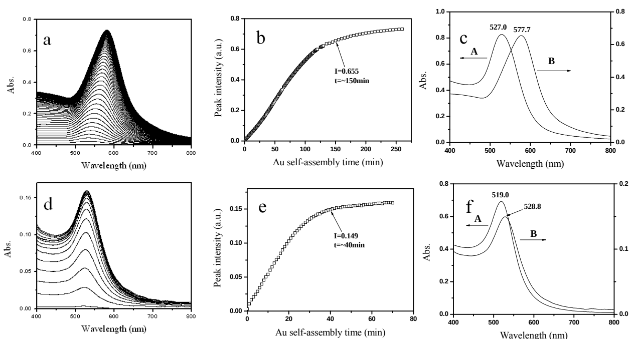
Figure 2. The absorption spectra of Au NP assembled films at different assembly time. (b) and (e); the LSPR peak intensity as a function of different assembly times. The assembly time is about 150 min for 48-nm Au and 39 min for 23-nm Au. (c) and (f); the absorption spectra before (A) and after the Au NP assembly (B). (a)-(c); 48-nm Au. (d)-(f); 23-nm Au.
