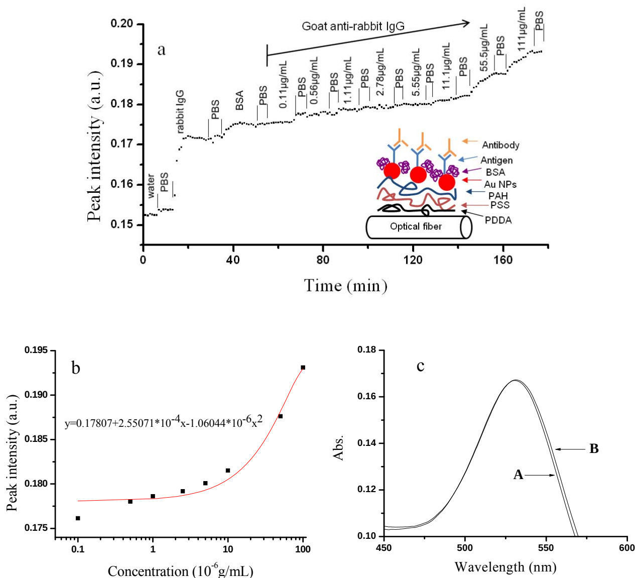
Figure 6. (a) The LSPR biosensing of different concentrations of goat anti-rabbit IgG (0.11–100 \mu\text{g/mL} ). (b) The standard curve of LSPR peak intensities with the antigen concentration of goat anti-rabbit IgG. (c) The LSPR sensing by using the present setup before (A) and after (B) 11.1 ng/mL of goat anti-rabbit IgG was added.
