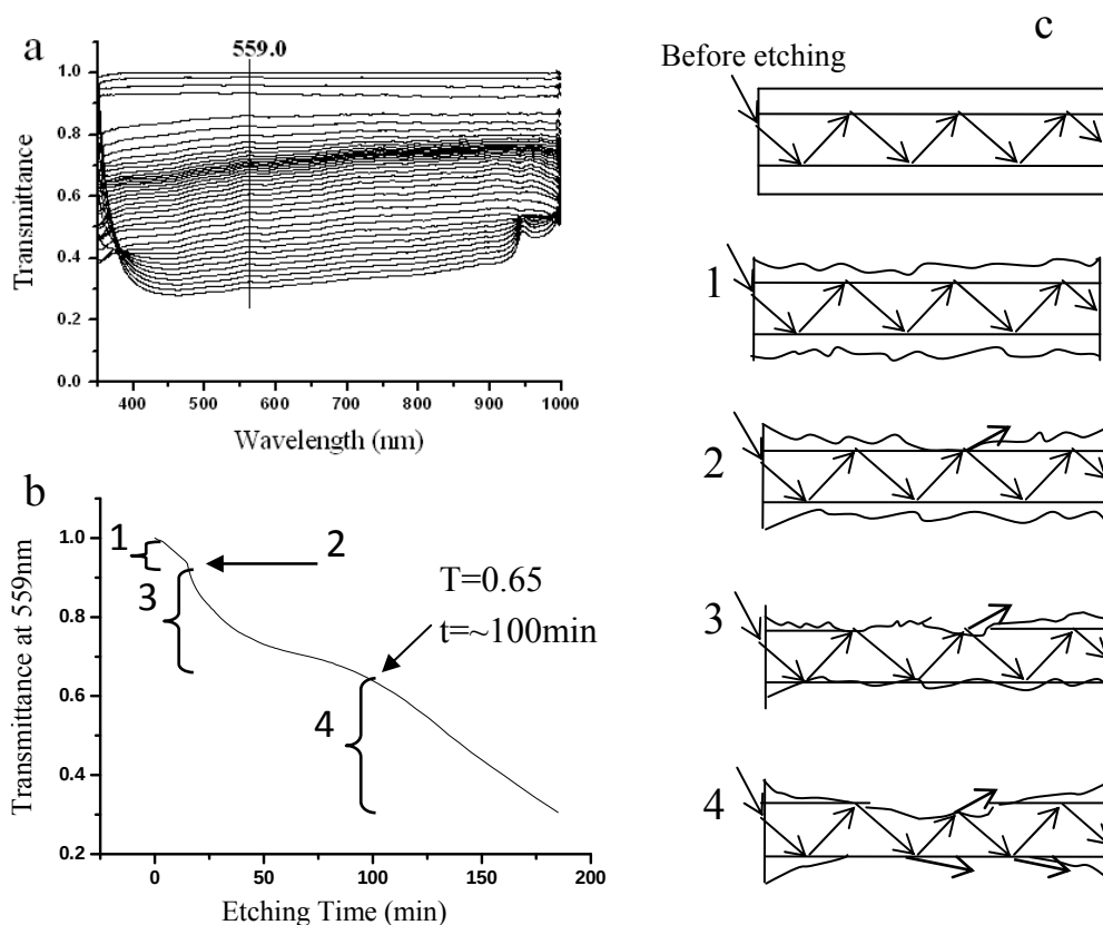
Figure 1. (a) The transmission spectra at different etching time. (b) The transmittance at 559.0 nm as a function of the HF etching time. (c) The schematic drawing of the fiber optic at different etching stages.
