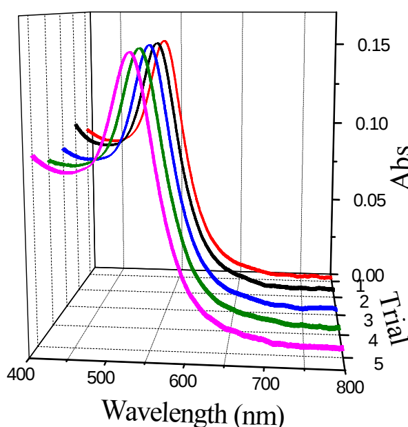
Figure 5. Comparison of the absorption spectra of the Au NP assembled films at different trials.
