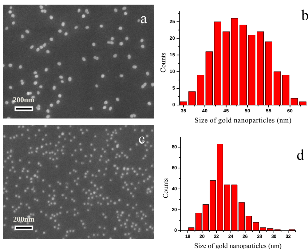
Figure 3. (a) and (c) The SEM images of the Au NP assembled films prepared with two different sizes of Au NPs; (b) and (d) The size distribution of Au NPs in (a) and (c). The diameter of (b) and (d) is 48 \pm 6 nm and 23 \pm 2 nm, respectively.
