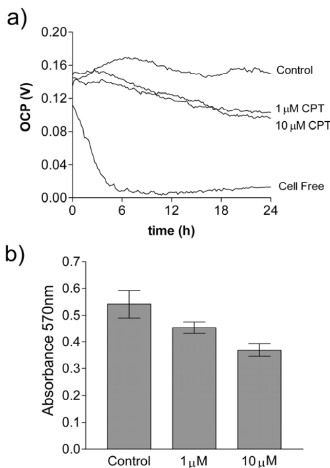
Figure 5. (a) Real-time electrochemical monitoring of the effect of camptothecin (CPT) on the OCP of HepG2 cells over 24 h ( n = 6 ). (b) MTT assay data (absorbance \pm SEM) from CPT treated HepG2 cells in parallel cultures after 24h ( n = 6 ).
