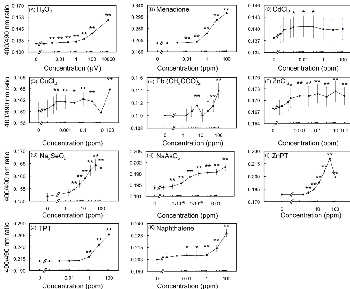
Figure 4. Concentration-response curves as shown by fluorescent ratiometric changes. Exposure to several concentrations of \text{H}_2\text{O}_2 (A), menadione (B), \text{CdCl}_2 (C), \text{CuCl}_2 (D), \text{Pb}(\text{CH}_3\text{COO})_2 (E), \text{ZnCl}_2 (F), \text{Na}_2\text{SeO}_3 (G), \text{NaAsO}_2 (H), \text{ZnPT} (I), TPT (J) and naphthalene (K). Each data point represents the ratiometric average of the dataset during 7 minutes (10–430 seconds) for a given concentration. Significant differences between control (concentration=0) and treated groups are indicated by * ( p < 0.05 ) and ** ( p < 0.01 ) using Dunnett's test followed by ANOVA. Error bars show \pm S.E.M. Error bars in panels A, B, I and J are too small to be seen.
