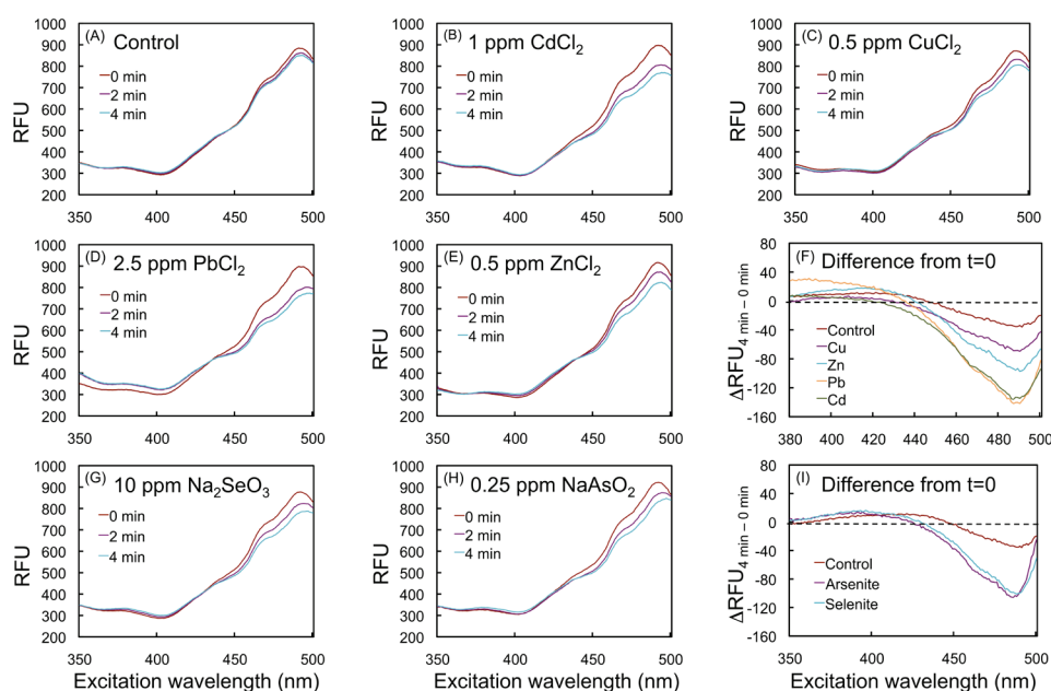
Figure 2. Spectroscopic analysis of E. coli -roGFP2 after induction of cellular oxidation by heavy metal compounds and oxyanions. Fluorescent excitation spectra of kinetic experiments after exposure of 4 minutes to water (A), 1 ppm \text{CdCl}_2 (B), 0.5 ppm \text{CuCl}_2 (C), 2.5 ppm \text{PbCl}_2 (D) and 0.5 ppm \text{ZnCl}_2 (E). Overall comparison among control and cations at 4 minutes after subtraction from 0 minute (F). Kinetic data obtained after 4 minutes exposure to 0.25 ppm \text{NaAsO}_2 (G) and 10 ppm \text{Na}_2\text{SeO}_3 (H). Overall comparison among oxyanions at 4 minutes after subtraction from 0 minute (I).
