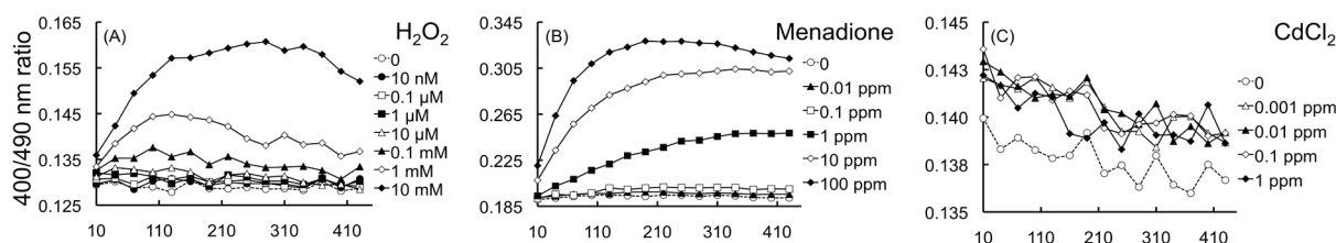
Figure 3. Multi-well ratiometric kinetic analysis of cellular oxidation using E. coli -roGFP2. Exposure to several concentrations of \text{H}_2\text{O}_2 (A), menadione (B), \text{CdCl}_2 (C), \text{CuCl}_2 (D), \text{Pb}(\text{CH}_3\text{COO})_2 (E), \text{ZnCl}_2 (F), \text{Na}_2\text{SeO}_3 (G), \text{NaAsO}_2 (H), \text{ZnPT} (I), TPT (J) and naphthalene (K). Each data point represents the average of six replicates. Measurements were made every 30 seconds during 7 minutes. Results shown correspond to a typical experiment, where each data point represents the quotient of the excitation fluorescence relative value at 400 and 490 nm.
