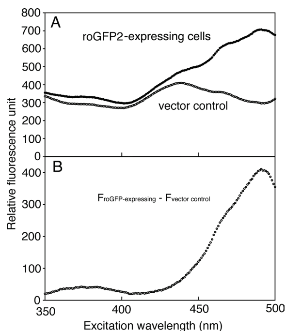
Appendix Figure 1. Fluorescence of roGFP2 expressed in E.coli cells. (A) fluorescence spectra of roGFP2-expressing cells (filled circle) and vector control (open circle), (B) subtraction of vector control from the roGFP2-expressing spectrum. Each data point was obtained within a 1 nm interval. The data presented shows the results from a single typical experiment of 3 replicates.
