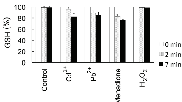
Figure 5. Effect of \text{Cd}^{2+} , \text{Pb}^{2+} , \text{H}_2\text{O}_2 and menadione on intracellular levels of GSH. Changes in concentration of GSH as quantified as described in Materials and methods are shown at 2 and 7 minutes after exposure to 0.1 ppm \text{CdCl}_2 , 1 ppm \text{Pb}(\text{CH}_3\text{COO})_2 , 1 ppm menadione and 1 mM \text{H}_2\text{O}_2 . Control corresponds to cells treated with \text{H}_2\text{O} . Six replicates were used for each dataset. Error bars indicate standard deviation.
