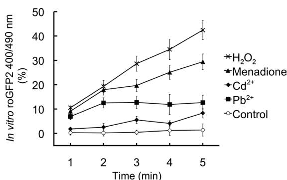
Figure 6. Effect of \text{Cd}^{2+} , \text{Pb}^{2+} , \text{H}_2\text{O}_2 and menadione and on roGFP2 in vitro . A 1.39 \mu\text{g}/\text{mL} solution of roGFP2 was exposed to 0.1 ppm \text{CdCl}_2 , 1 ppm \text{Pb}(\text{CH}_3\text{COO})_2 , 1 ppm menadione and 1 mM \text{H}_2\text{O}_2 . Changes in 400/490 nm fluorescence ratio were monitored for 5 minutes with a multi-well plate reader and expressed in percentage compared to the value at t = 0 minute. Three replicates were used for each dataset and error bars indicate standard deviation.
