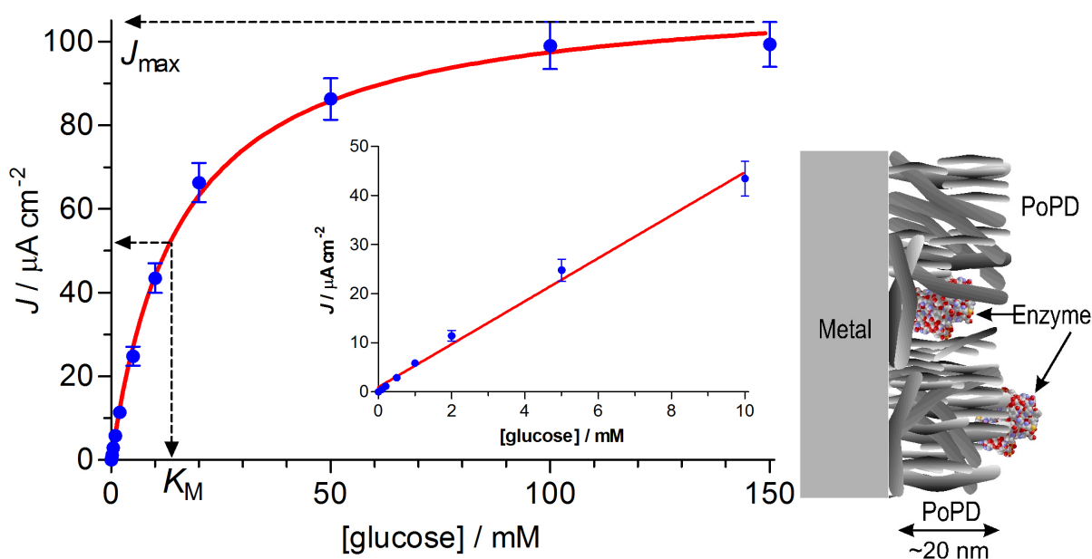
Figure 1. Sample steady-state calibration data and nonlinear regression analysis for the biosensor design, Pt C /PoPD-GOx [Equation (4), R^2 = 0.998 , n = 8 ; left ], illustrating the graphical significance of the Michaelis-Menten constants, J_{\max} and K_M . The linear region slope (LRS) was obtained using linear regression up to 10 mM glucose ( R^2 = 0.996 , n = 8 ; left inset ), and represents the most suitable measure of analytical sensitivity of each biosensor design to enzyme substrate (see Table 1). Schematic representation of the PEC configuration for the same Pt C /PoPD-GOx design ( right ), illustrating trapped GOx (~8 nm diameter) in the PoPD layer deposited by the precipitation of insoluble chains formed during the electropolymerization of monomer solution containing the enzyme.
