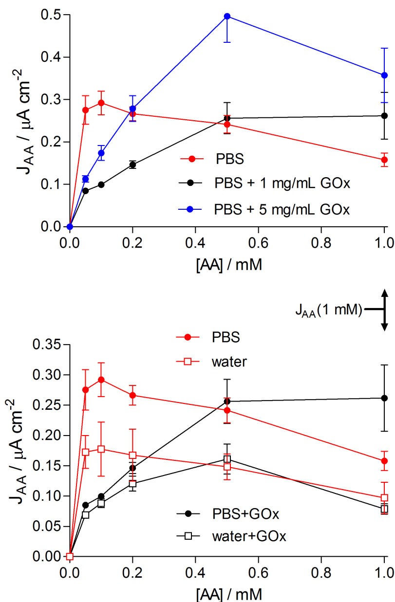
Figure 2. Averaged steady-state AA calibrations for Pt C /PoPD and Pt C /PoPD-GOx electrosynthesized in 300 mM oPD solution made with either PBS*, PBS + GOx (1 mg mL -1 , n = 4 ), PBS+GOx (5 mg mL -1 , n = 8 ), distilled water*, or water+GOx (1 mg mL -1 , n = 6 ). The concentration of GOx for the bottom graph was 1 mg mL -1 . *The GOx-free data were taken from the literature [38] for comparison.
