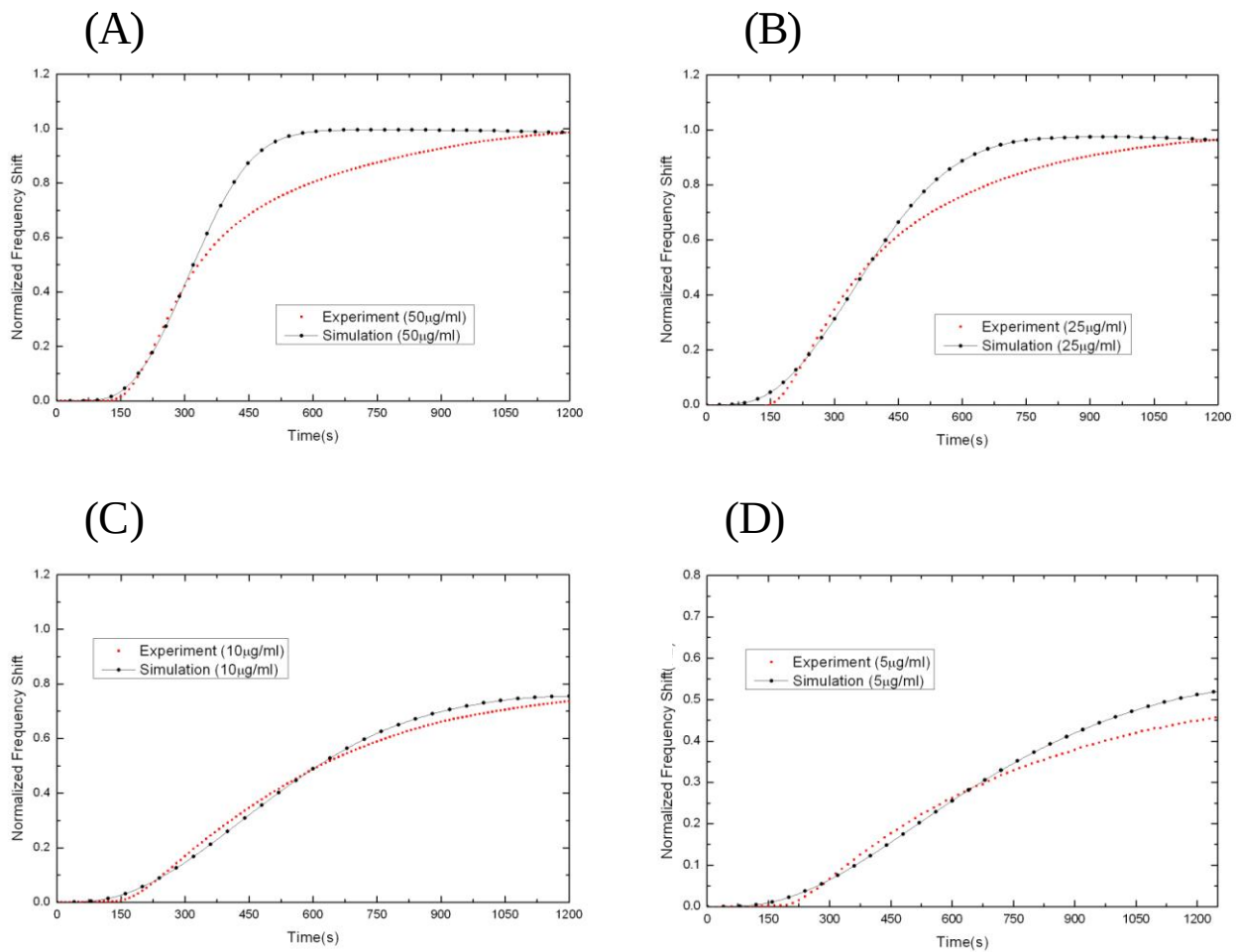
Figure 6. The normalized experimental and simulated binding reaction curves for the 800 \mu\text{L} supplement volume. Here the concentrations of the Anti-Human IgG1 solution are (A) 50 \mu\text{g/mL} , (B) 25 \mu\text{g/mL} , (C) 10 \mu\text{g/mL} , and (D) 5 \mu\text{g/mL} .
