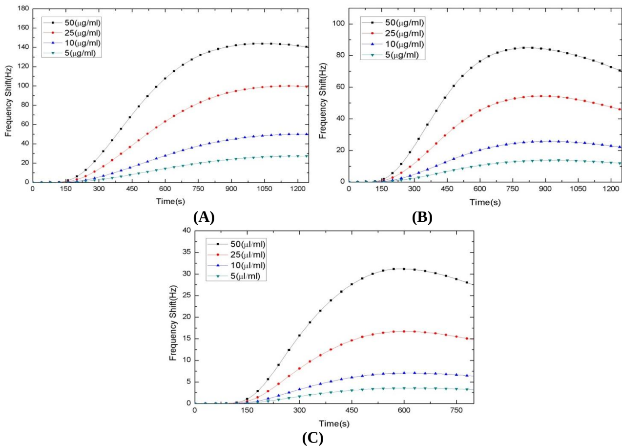
Figure 4. Simulated binding reaction curves. The supplement volume of the Anti-Human IgG1 solution is (A) 800 \mu\text{L} (B) 500 \mu\text{L} and (C) 100 \mu\text{L} .
