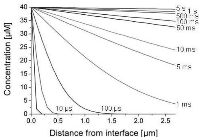
Figure 4. Diffusion gradients—Calculated concentration gradients of methanethiol across the liquid phase at selected time intervals after initial contact of the sample gas with the biosensor.
