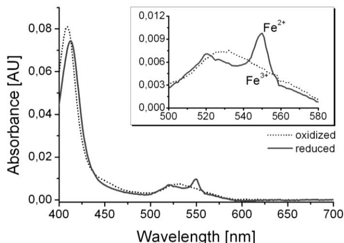
Figure 3. UV-spectra of cytochrome c—typical spectra of cytochrome c with three absorbance peaks of its reduced form ( \text{Fe}^{2+} ) at 550 nm, 521 and 414 nm (solid line) and two peaks of its oxidized form ( \text{Fe}^{3+} ) at 530 nm and 408 nm (dotted line). The inset shows an expanded view of the spectra between 500 and 580 nm.
