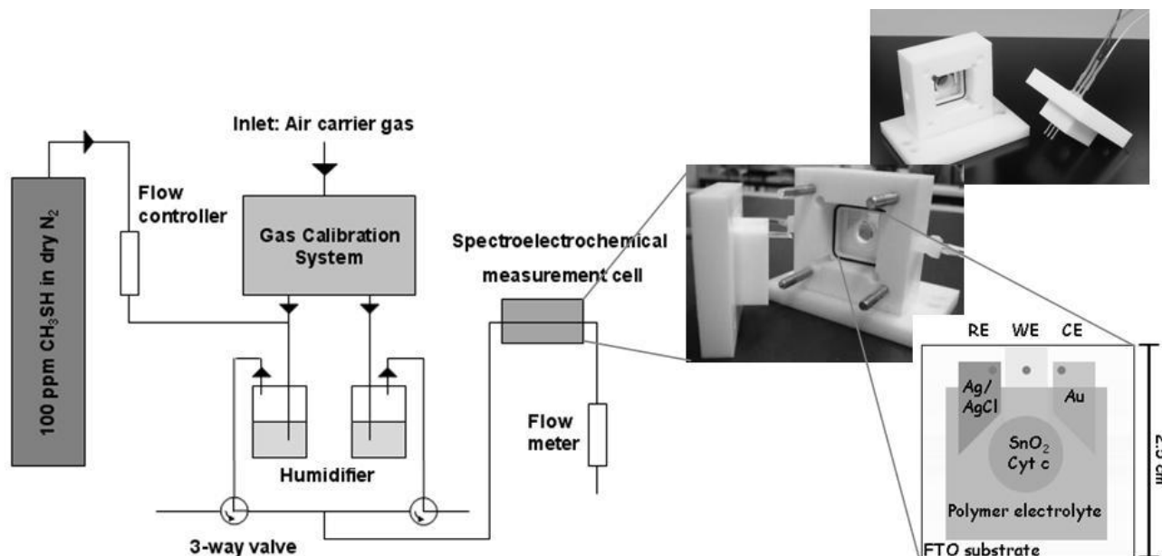
Figure 1. Gas-measurement set-up—A mixture of 100 ppm methanethiol in nitrogen was taken from a pressurized gas bottle. The gas was humidified and could stream into the gas-tight measurement cell. Valves allowed switching between test gas (humidified air with methanethiol) and reference gas (humidified air without methanethiol). The images show the gas-tight spectroelectrochemical measurement cell and a schematic picture of the biosensor.
