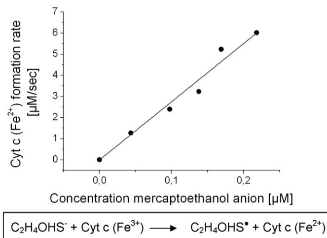
Figure 5. Formation rate of cytochrome c ( \text{Fe}^{2+} ) in liquid phase plotted vs. mercaptoethanol anion concentrations—Cytochrome c was adsorbed onto \text{SnO}_2 on FTO and mercaptoethanol was dissolved in buffer solution. Mercaptoethanolate reduced the oxidized cytochrome c and lead to increased absorption at 550 nm. Changes in concentration of cytochrome c were calculated from changes in light absorption via Lambert-Beer's law.
