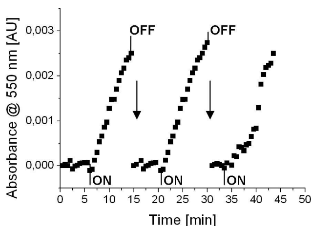
Figure 6. Gas biosensor measurements—with a cytochrome c modified electrode and gaseous methanethiol. The changes in absorbance at 550 nm are plotted versus the time of the experiment. The moments when reference gas was switched to methanethiol-containing gas sample are marked with “ON”, whereas “OFF” indicates switching from methanethiol-containing gas sample to reference gas. The vertical arrow indicates electrochemical oxidation of cytochrome c (60 s, +100 mV vs. Ag/AgCl) to reset to baseline absorbance and to prepare the biosensor for the next exposure of gas sample.
