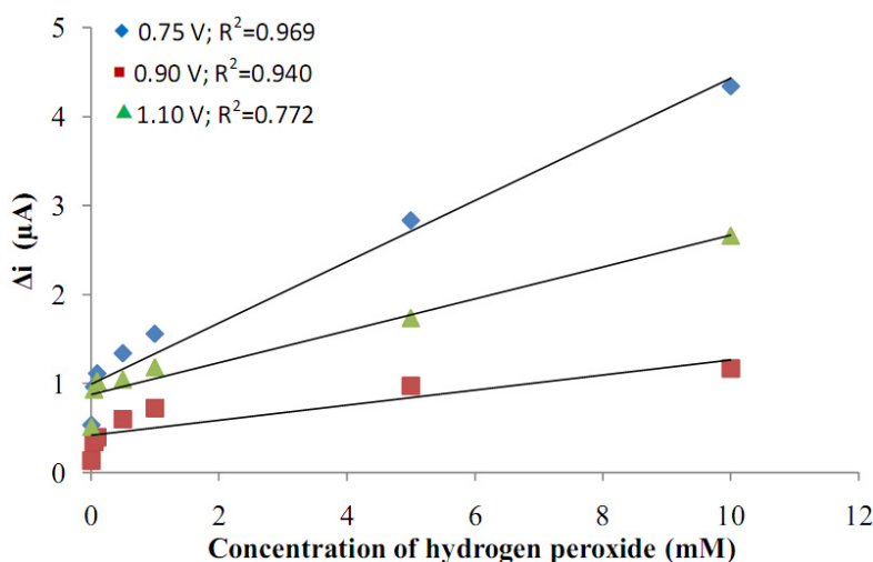
Figure 1. Potential of Pt/Pani-Pvs film vs. \text{H}_2\text{O}_2 concentration.
