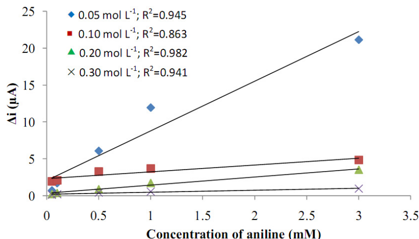
Figure 2. Effect of aniline concentration on the response of the Pt/Pani-Pvs electrode to hydrogen peroxide.
