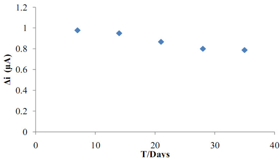
Figure 11. Storage stability of the biosensor (in pH 7.5 phosphate buffer, at 0.4 V operating potential, 25 °C and 1.0 \times 10^{-5} M substrate concentration).
