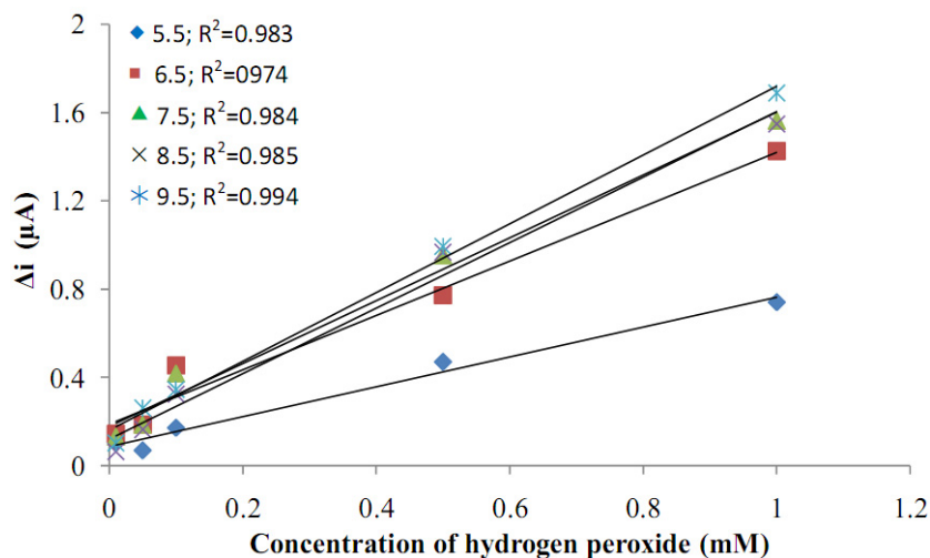
Figure 5. Effect of pH on the response of the Pt/Pani-Pvs electrode to hydrogen peroxide.
