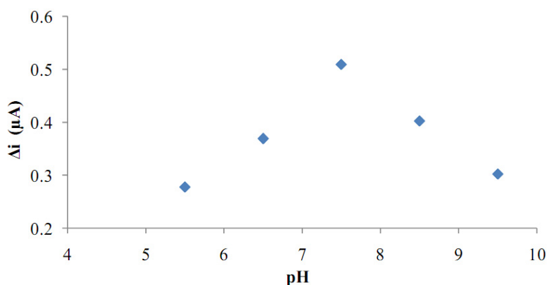
Figure 6. The effect of pH on the response of the biosensor (at 25 °C, 1.0 \times 10^{-5} M glucose at 0.4 V operating potential).
