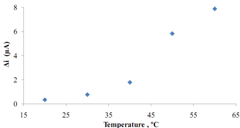
Figure 7. The effect of temperature on the response of the biosensor (at pH 7.5, 1.0 \times 10^{-5} M glucose at 0.4 V operating potential).
