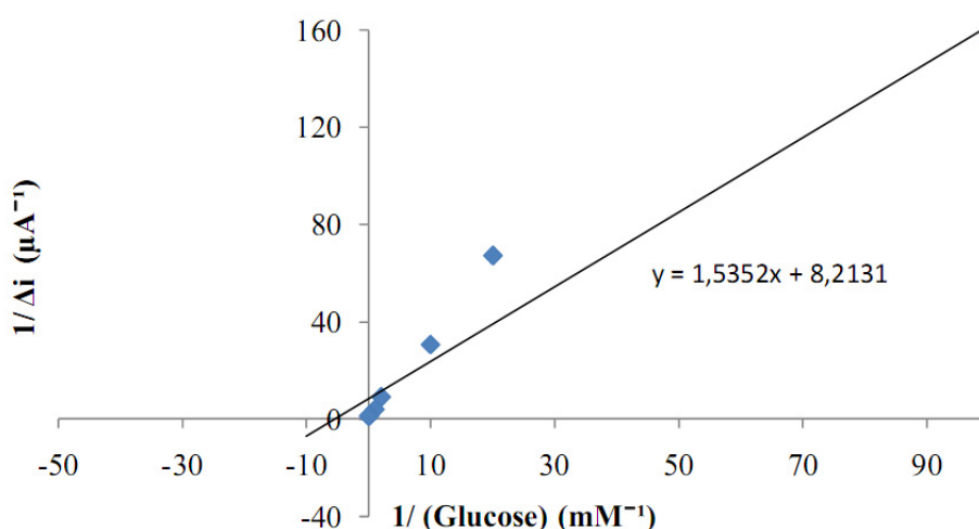
Figure 9. The effect of glucose concentration upon the amperometric response of the biosensor (Lineweaver-Burk plot, in pH 7.5 phosphate buffer and at a 0.4 V operating potential, 25 °C).
