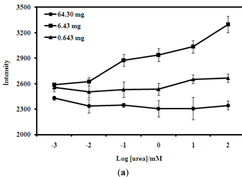
Figure 6. (a) The effects of the amount of acrylic microspheres coated onto a film on the urea biosensor response (measured at fixed time analysis 10 min); and (b) The effects of exposure time to urea on the response of the urea biosensor (fixed amount of coated microspheres).
