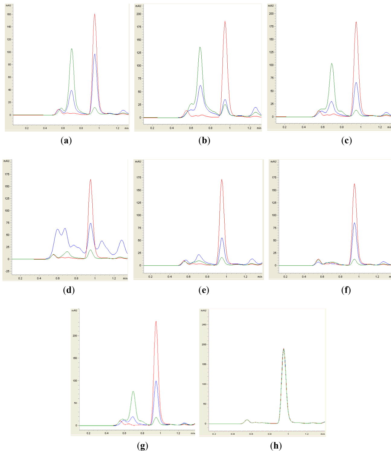
Figure 2. RRLC analysis of C10-HSL degradation. Residual C10-HSL (with elution time of 0.95 \pm 0.02 min), after degradation for 0 h (red), 3 h (blue) and 24 h (green), was monitored at 210 nm. Degradation of C10-HSL was depicted by the reduction of milli-absorbance unit (mAU) in the chromatogram. Samples containing BT1 (a), BT2 (b), BT4 (c), BT6 (d), BT8 (e), BT9 (f) and B. cereus (g) showed significant degradation of C10-HSL. PBS buffer (h) was used as the negative control for the analysis.
