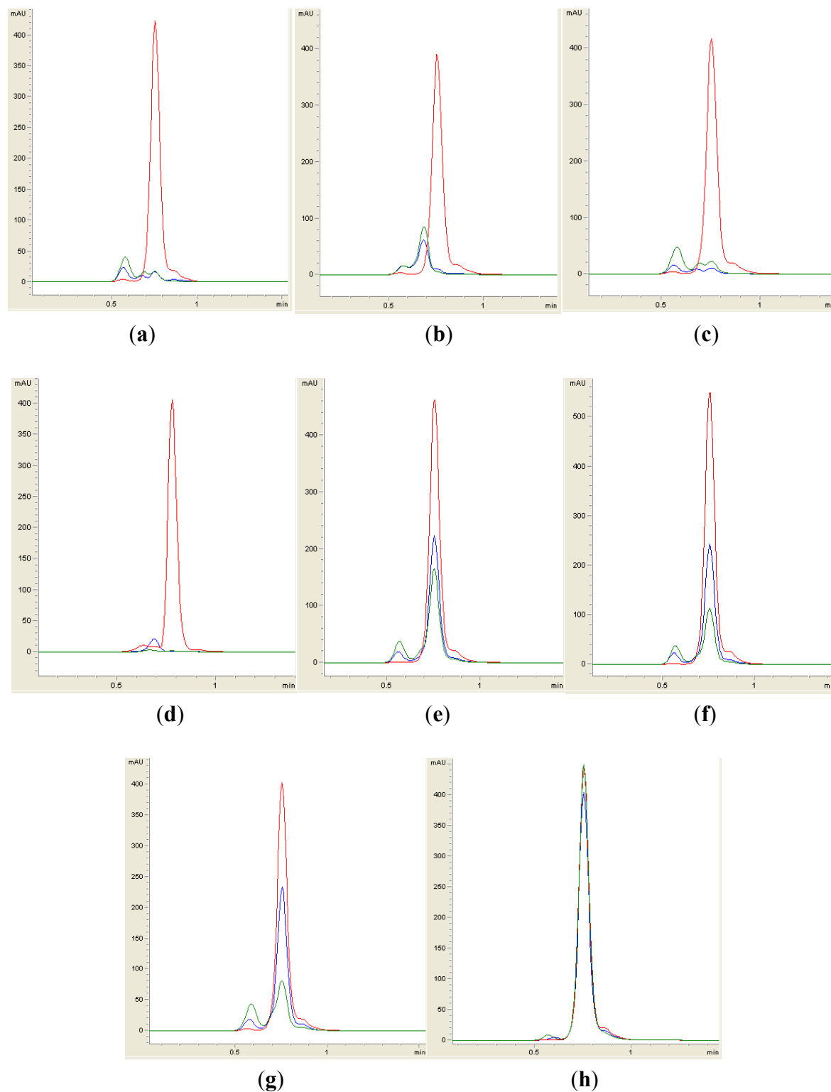
Figure 4. RRLC analysis of pC-HSL degradation. Residual pC-HSL (with elution time of 0.75 \pm 0.01 min), after degradation for 0 h (red), 12 h (blue) and 24 h (green), was monitored at 306 nm. Degradation of pC-HSL was depicted by the reduction of milli-absorbance unit (mAU) in the chromatogram. Samples containing BT1 (a), BT2 (b), BT4 (c), BT6 (d), BT8 (e), BT9 (f) and B. cereus (g) showed degradation of pC-HSL. E. coli TOP10 (h) was used as the negative control.
