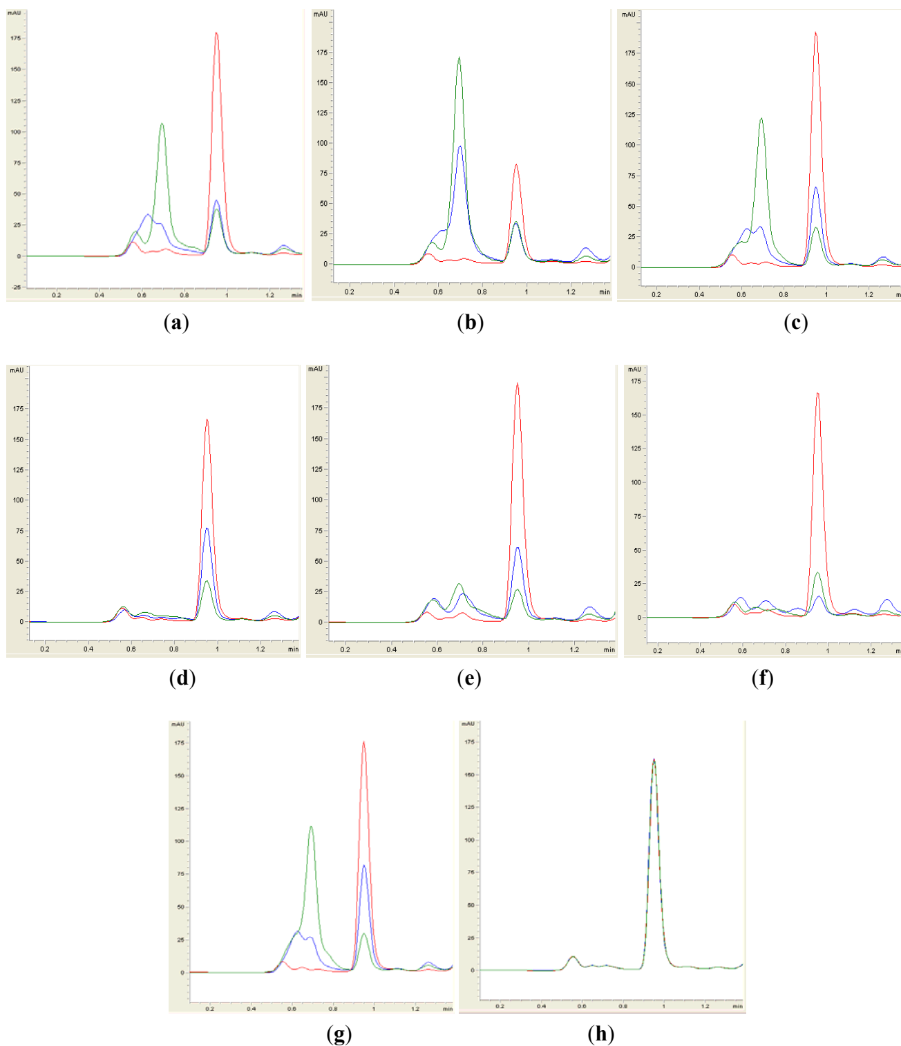
Figure 3. RRLC analysis of 3-oxo-C12-HSL degradation. Residual 3-oxo-C12-HSL (with elution time of 0.95 \pm 0.02 min), after degradation for 0 h (red), 3 h (blue) and 24 h (green), was monitored and degradation of 3-oxo-C12-HSL was observed for all bacteria tested, such as BT1 (a), BT2 (b), BT4 (c), BT6 (d), BT8 (e), BT9 (f) and B. cereus (g). PBS solution (h) was the negative control for the analysis.
