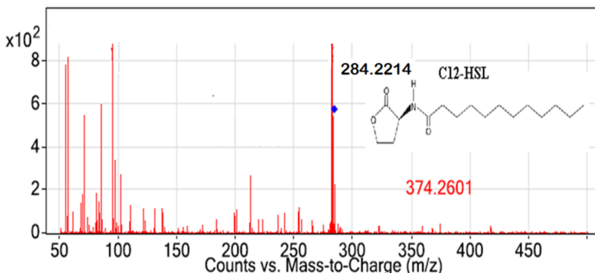
Figure 5. ESI-MS spectrum of C12-HSL ( m/z 284.2214, 7.708 min).
