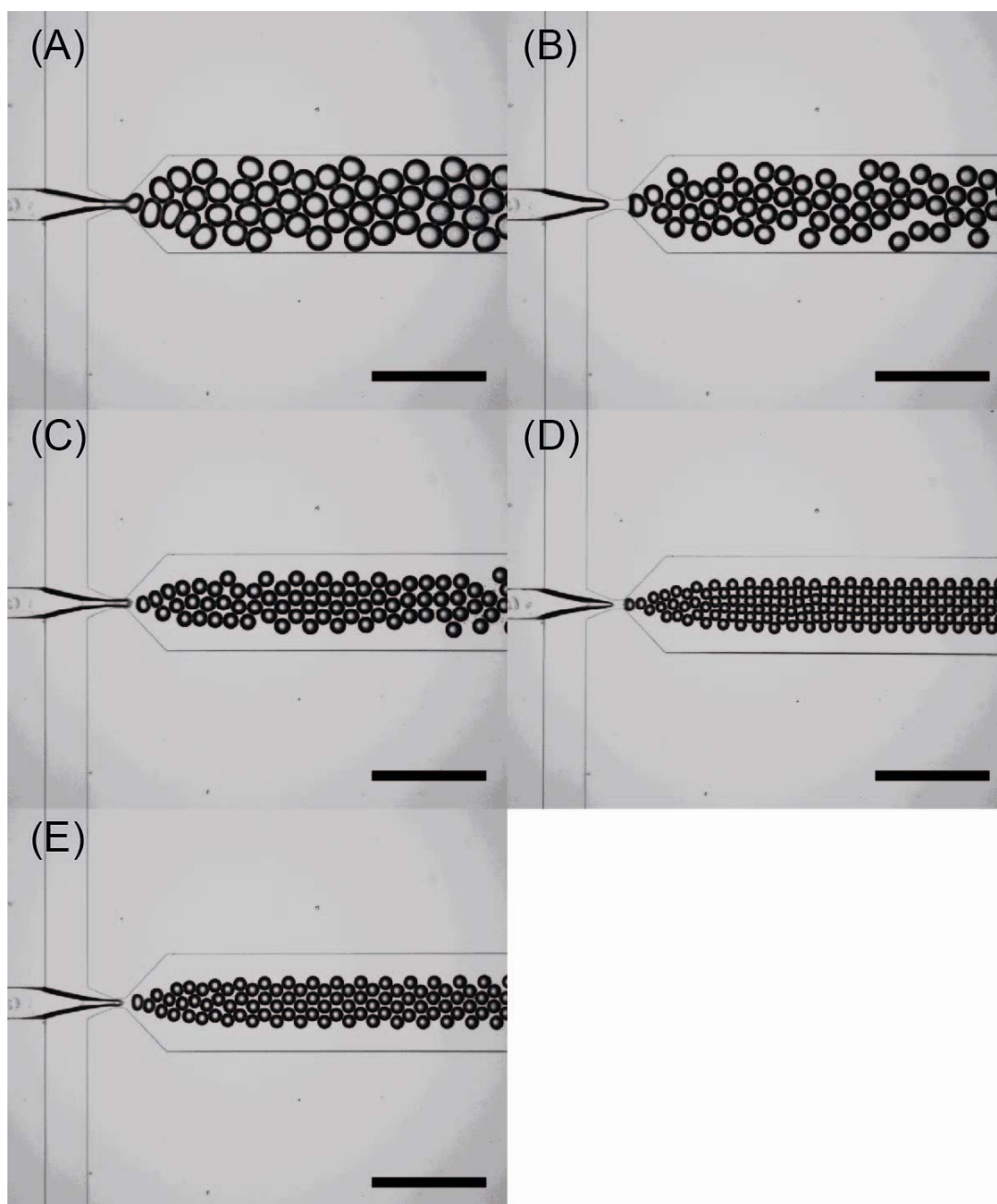
Figure S4. Photomicrographs showing the droplets of different sizes at the fixed DP (3 \mu\text{L}/\text{min} ) with five different flow rates of CP. (A) Q_{\text{CP1}} = 1 \mu\text{L}/\text{min} ; (B) Q_{\text{CP2}} = 2 \mu\text{L}/\text{min} ; (C) Q_{\text{CP3}} = 3 \mu\text{L}/\text{min} ; (D) Q_{\text{CP4}} = 4 \mu\text{L}/\text{min} ; (E) Q_{\text{CP5}} = 5 \mu\text{L}/\text{min} . All scale bars are 500 \mu\text{m} .
