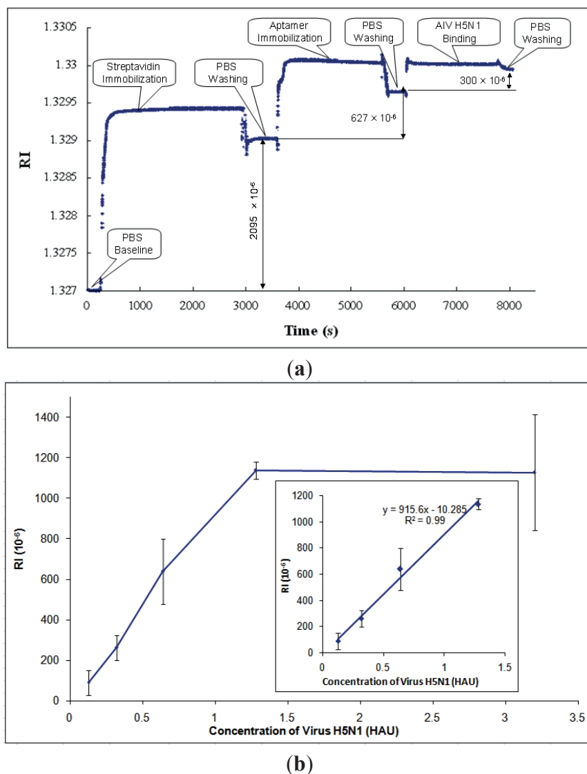
Figure 5. Detection of AIV H5N1 using SPR aptasensor: (a) A typical response curve of the SPR aptasensor to the surface modification and AIV H5N1 detection; (b) Calibration curve for AIV H5N1 detection (all tests were repeated three times).
