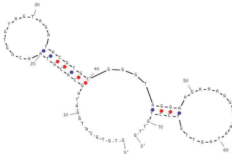
Figure 1. Sequence and predicted secondary structure of the aptamer used in this study.
