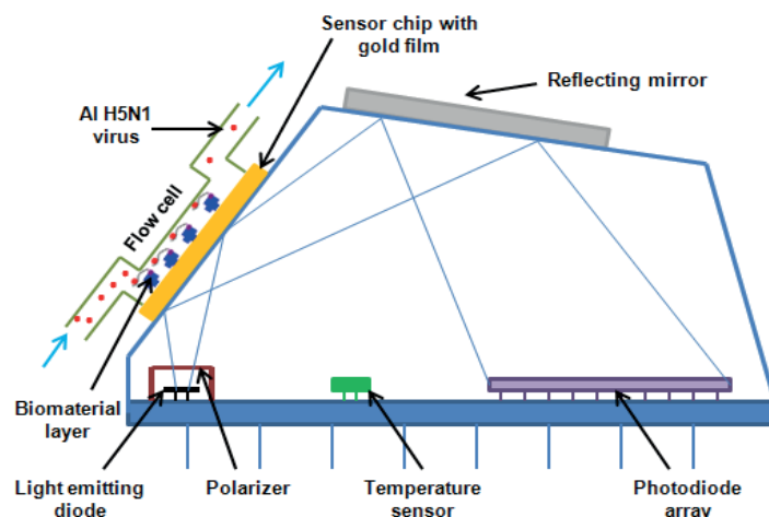
Figure 2. The configuration for measuring AIV using the portable SPR aptasensor.
