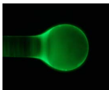
Figure 2. Fluorescent image of the sample anti-mouse-IgG.
