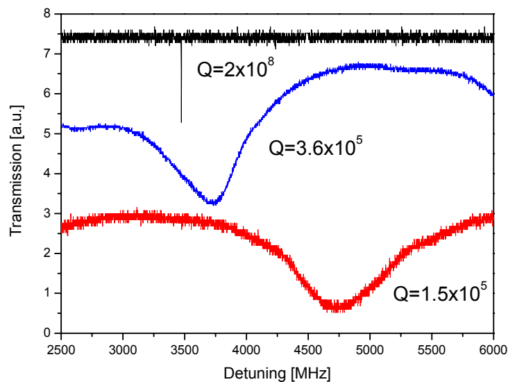
Figure 3. Measured Q factor of the NT sample (black line), of a covalent binding of IgG (blue line) and an IgG/anti-IgG interaction (red line).
