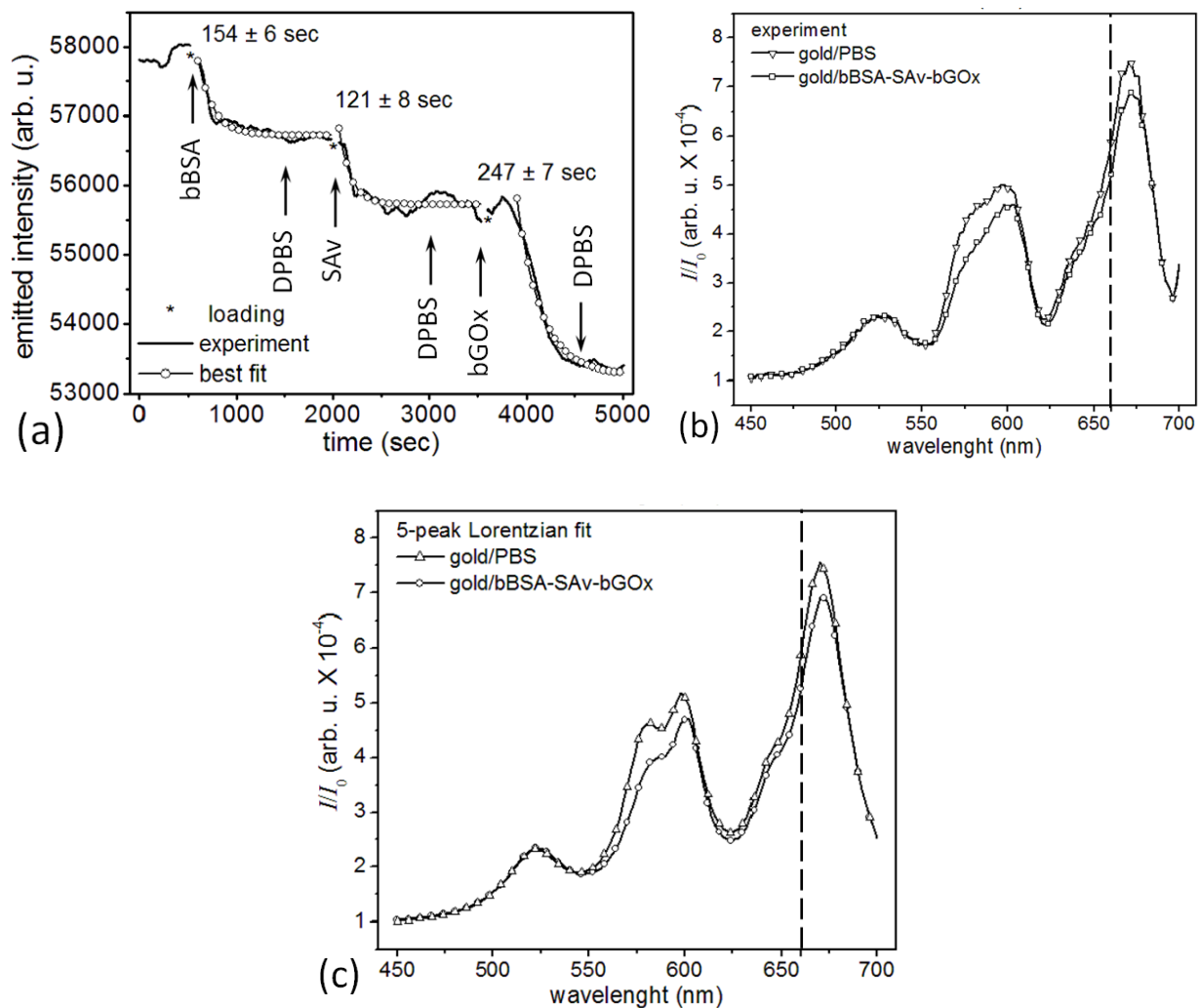
Figure 6. (a) Monitoring the successive binding of three molecular layers to a microsensor: a microsensor's emitted-light intensity at 660 nm (dashed line in Figure 6(b) and 6(c)) during: (i) covalent binding of 10- \mu M bBSA solution to the microsensor's bare-gold surface, (ii) subsequent binding of a 10- \mu M SAv solution to the microsensor-bound bBSA, (iii) subsequent binding of a 100-nM bGOx solution to the microsensor-bound bBSA-SAv complex. (○) exponential-decay best-fits to the emitted-light intensities: R^2(\text{bBSA}) = 0.91 , R^2(\text{SAv}) = 0.78 , R^2(\text{bGOx}) = 0.97 . The sample flow rate was \approx 0.2 nL/s and the solution temperature was 24.0 \pm 0.1 °C. *No signal was recorded during sample loading. (b) Spectra of a microsensor consisting of a \varnothing 780 polystyrene nanosphere covered uniformly with a \approx 150 nm gold film and excited with white light from a microscope illuminator (0.3 NA), showing the four main visible microcavity resonances (i) ( \nabla ) spectrum for the bare-gold microsensor in DPBS, (ii) ( \square ) spectrum for the microsensor after deposition of bBSA-SAv-bGOx. (c) Multi-peak Lorentzian fits of the spectra in Figure 6(b): (i) ( \triangle ) for the bare-gold microsensor in DPBS, R^2(\text{DPBS}) = 0.99 , and (ii) (○) for the microsensor after deposition of bBSA-SAv-bGOx R^2(\text{bBSA-SAv-bGOx}) = 0.99 .
