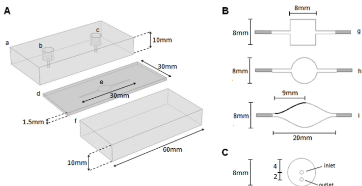
Figure 3. Experimental flow cell construction ( A ): (a) PMMA top block with (b) inlet and (c) outlet holes. Inlet and outlet accommodate \frac{1}{4} "-28 threaded nuts at the top and feature 1mm openings at the fluid inlet/outlet point; (d) PTFE gasket with (e) 30mm cut-out flow domain section; (f) PMMA base block. Bolt holes used to secure the flow cell unit are not shown for clarity. ( B ) Flow domain channel geometries: (g) square cell; (h) circular cell; (i) iCell (the heavier line of the iCell shows the curve shape upon which this flow cell is profiled); unshaded area indicates region of interest for flow analysis. ( C ) Modeled impinging jet flow cell geometry. The height of flow domains for (b) and (c) is 1.5 mm.
