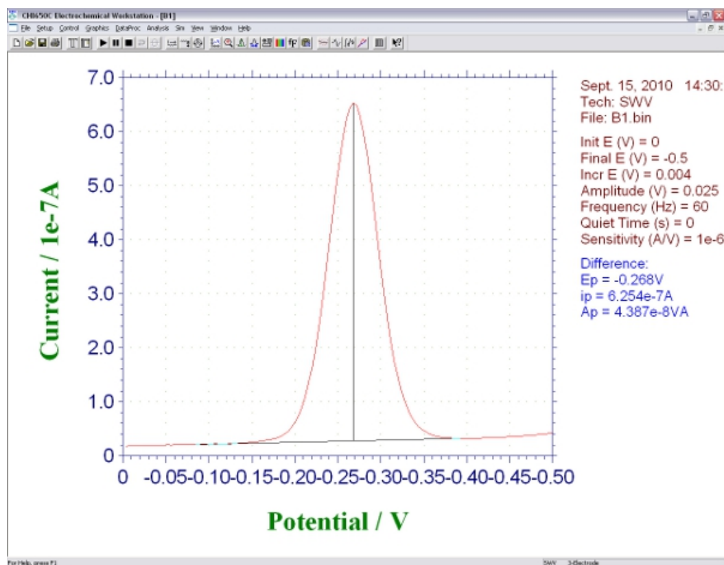
Figure 2. Screen shot showing the signal produced by an E-DNA biosensor during square wave voltammetry.
