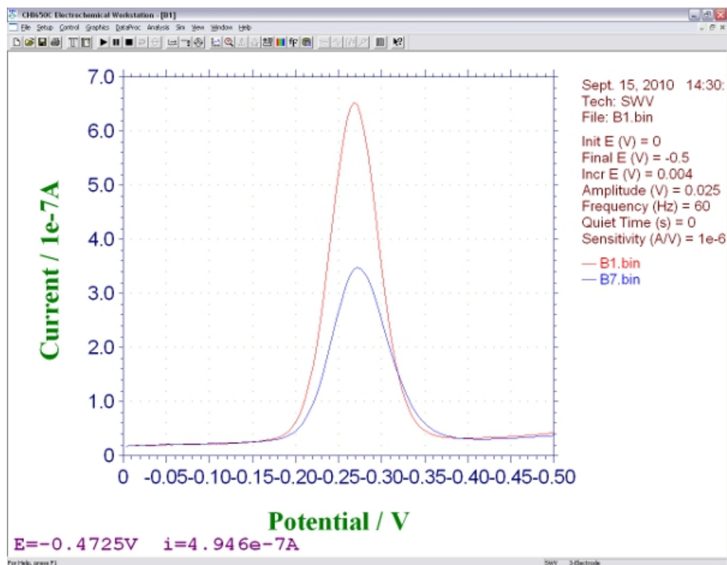
Figure 3. Screen shot showing the signals produced by an E-DNA biosensor during square wave voltammetry, before and after hybridization with an analyte.
