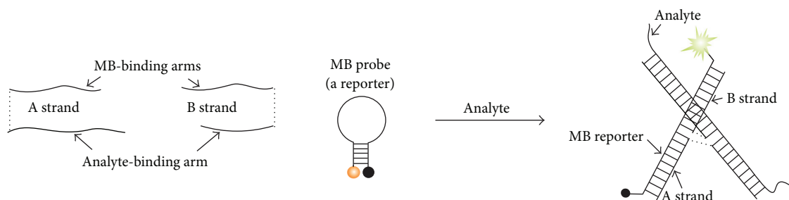
FIGURE 6: Using a universal MB (UMB) probe as a part of tricomponent X sensor for recognition of specific DNA or RNA sequences [98, 108]. Adaptor A and B strands hybridize to both analyzed sequence and a universal near-optimal MB probe reporter to form fluorescent tetrapartite complex. Triethylene glycol linkers (TEG) that connect the MB-binding arms with the analyte-binding arms are shown as dashed lines.
